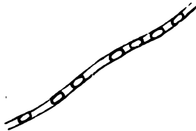
FIG. 111.—SPORES OF BACILLUS ANTHRACIS UNSTAINED, \times 1500 .
